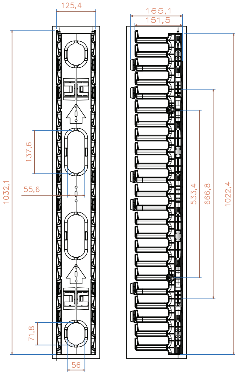
Vertical Cable Manager w/ removable-hinged cover, 200 cables 22.5RU, Front only
