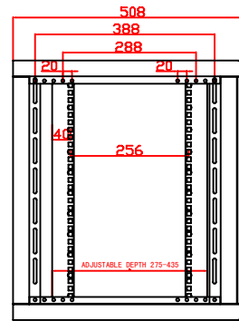
SIDEVIEW WITH PANEL REMOVED
