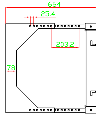
SIDE AT MAXIMUM DEPTH
