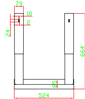
TOP AT MAXIMUM DEPTH
