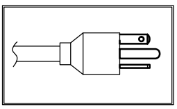
NEMA 5-20P 20A,120V MOLDED ON PLUG
